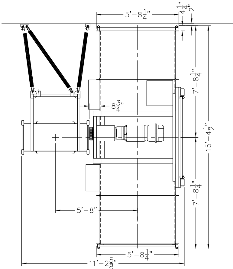
CAR LAYOUT - US8000S-DUAL TWR SCALE: 1/4" = 1'-0"
