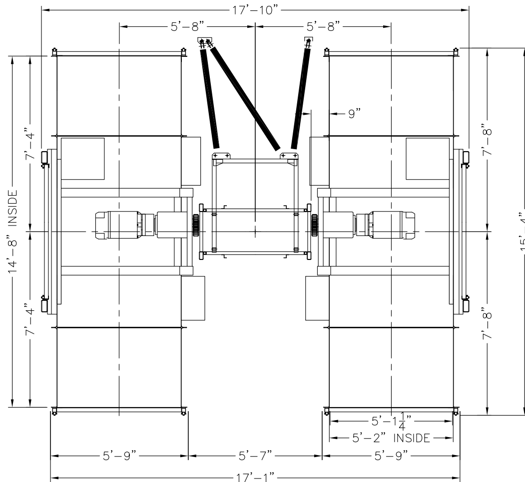
CAR LAYOUT - US8000D STD.
